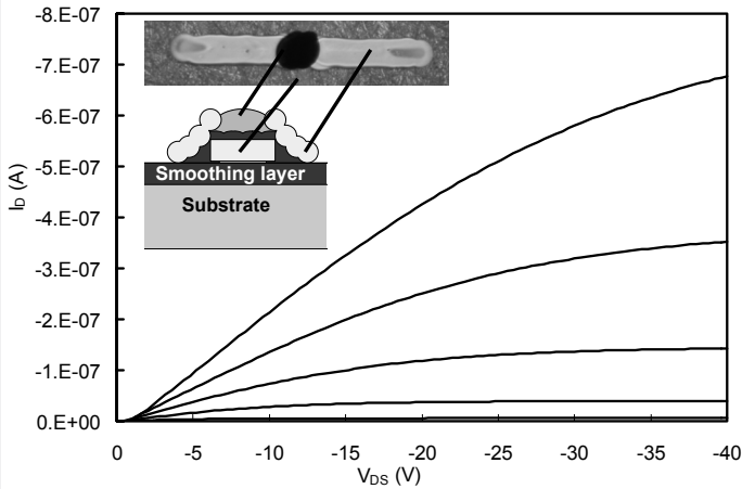
Figure 15.3.1: Micrograph, schematic cross-section, and electrical characteristics of printed TFT (W/L=120µm/45µm).
