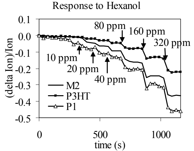
Figure 15.3.2: Response of a 3-element sensor (with an oligothiophene, M2, a polythiophene, P3HT, and a pentacene P1) to hexanol vapors, showing ppm level sensitivity.
