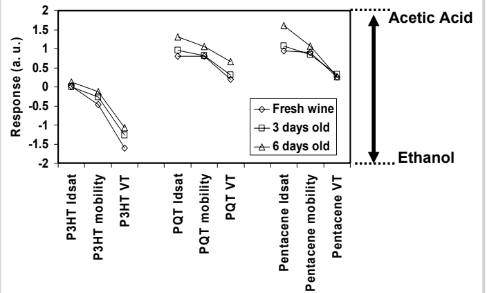
Figure 15.3.6: Sensing of wine spoilage using a 3-element array. The transistor channels are polythiophene (P3HT), polyquaterthiophene (PQT), and pentacene respectively.
